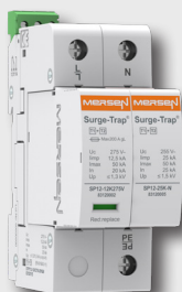
Combined Type 1 & 2
