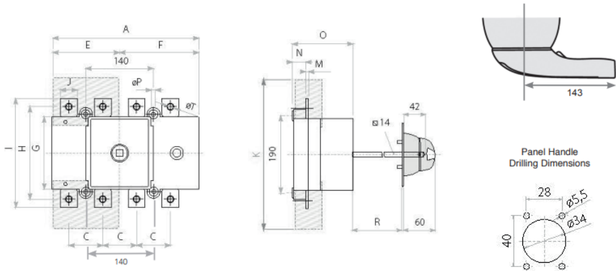
Dimensions (mm)
