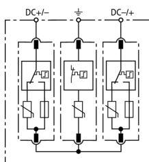
Basic circuit diagram DG M YPV SCI 1000
