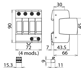
Dimension drawing DG M TT ... FM
