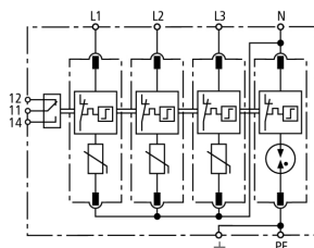
Basic circuit diagram DG M TT ... FM
