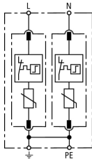
Basic circuit diagram DG M TN ...
