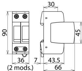
Dimension drawing DG M TN ...
